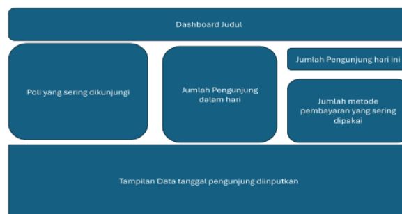
Gambar 3. Mockup Dashboard
